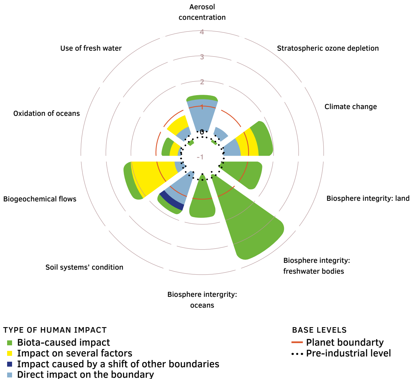
Figure 2. Planetary boundaries: assessing the current state (Source [Lade, Steffen, de Vries et al., 2020])
